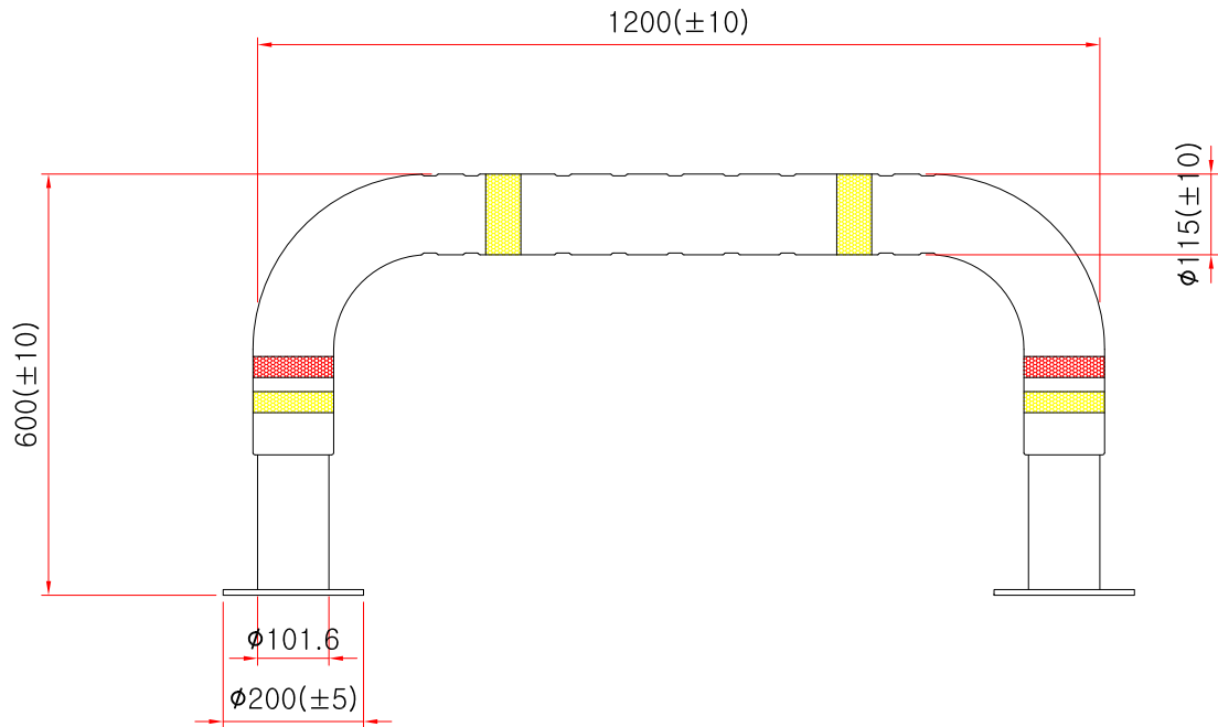
SIDE ELEVATION SCALE : NONE
