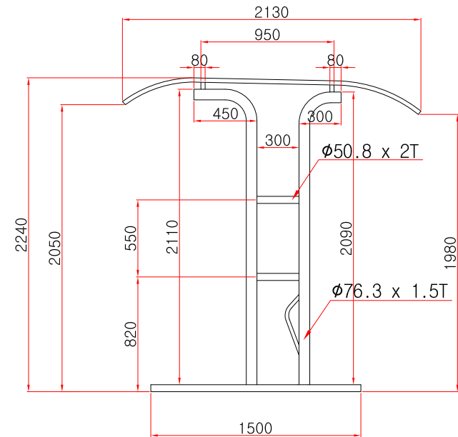
SIDE ELEVATION SCALE : NONE
